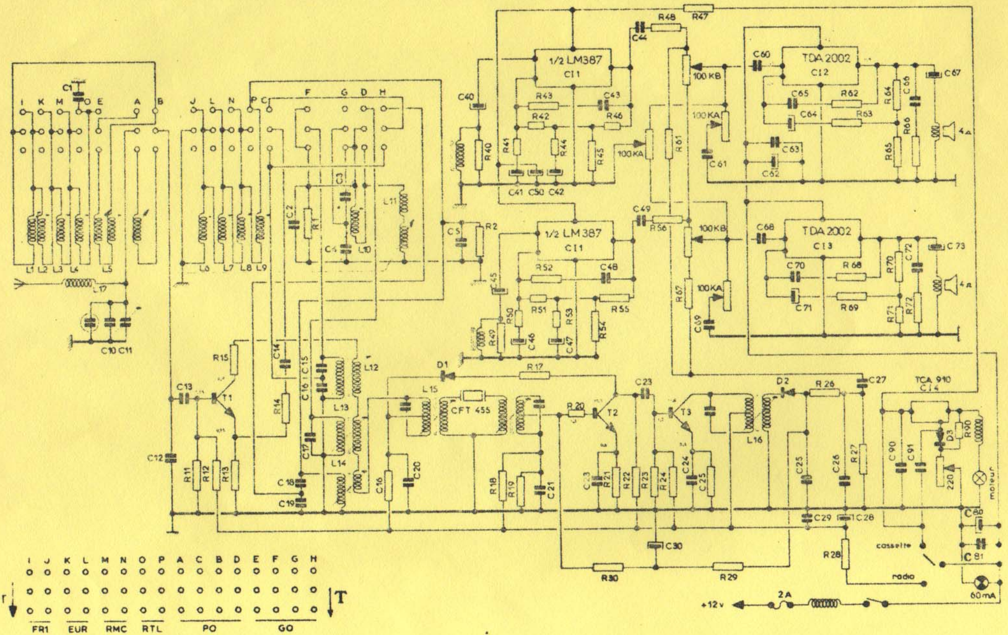
SCHEMA THEORIQUE AUTO-RADIO CASSETTE STEREO PO GO. 4 Prerogies "NORMANDIE" CONCEPTO
