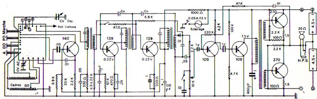
Pygmy-Radio
